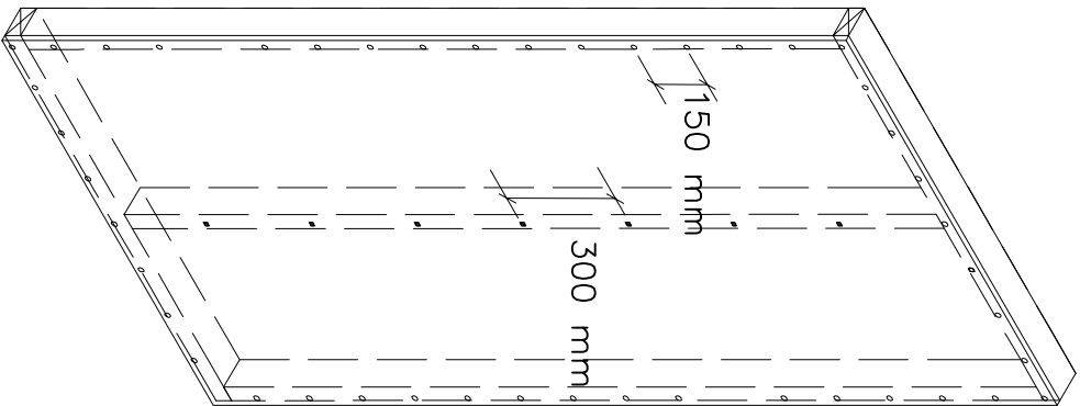
Ecoply® fastened in vertical plane
